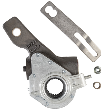
Slack Adjusters - Haldex (School Bus)
