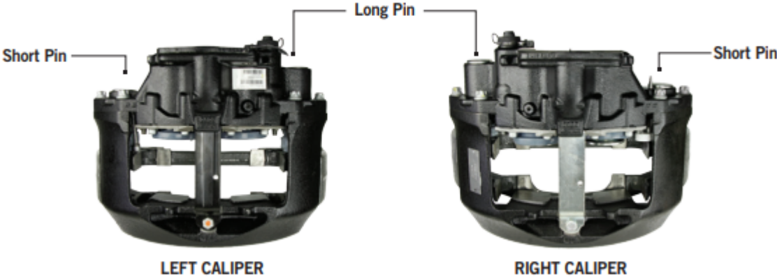
AXIAL MOUNT
