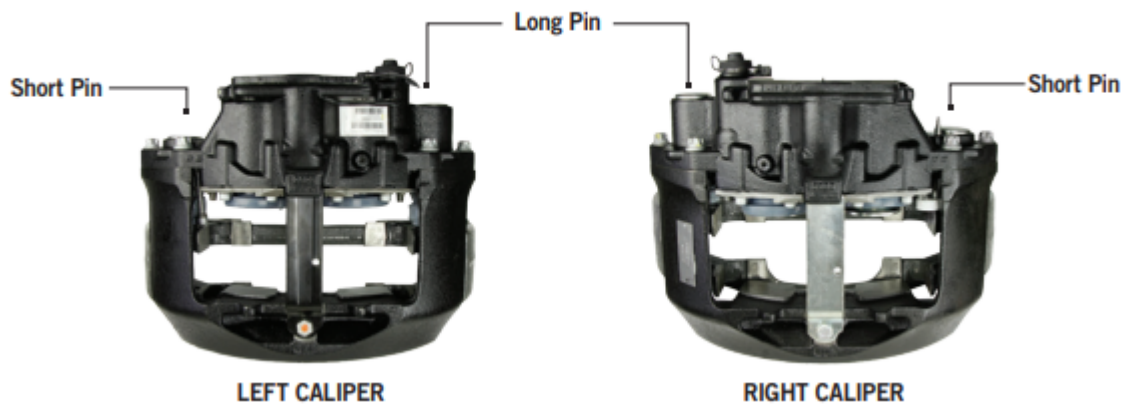
AXIAL MOUNT
