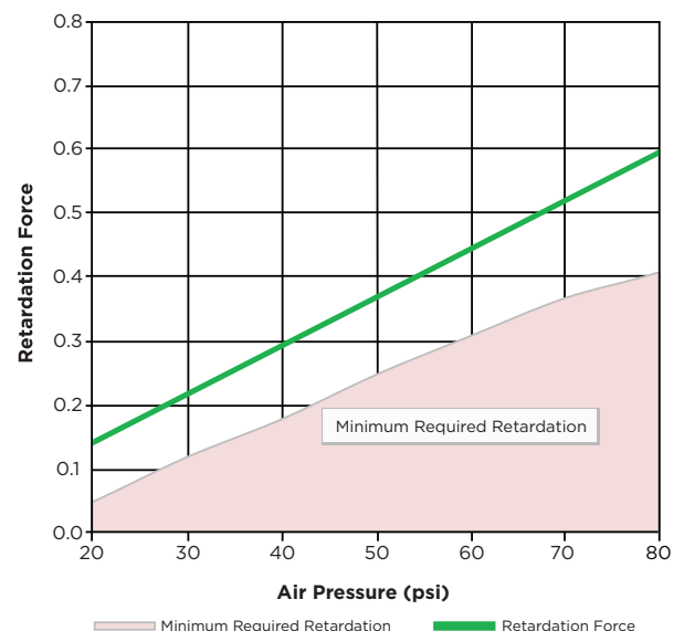
50 MPH Retardation
