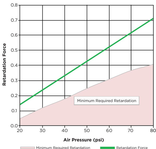
50 MPH Retardation
